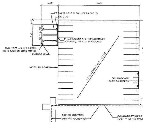
FLOOR FRAMING PLAN 1/4" = 1'-0"
