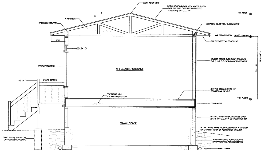
'A' SECTION 1/2" = 1'-0"
