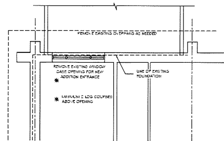
DEMO PLAN 1/4" = 1'-0"
